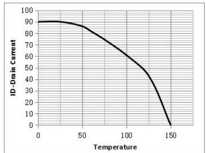
Fig.10 ID-Junction Temperature
